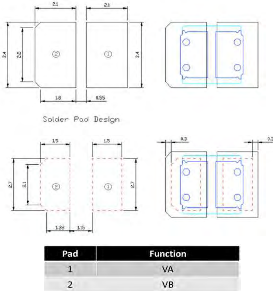
Figure 9 Recommended Solder Pad Dimensions
