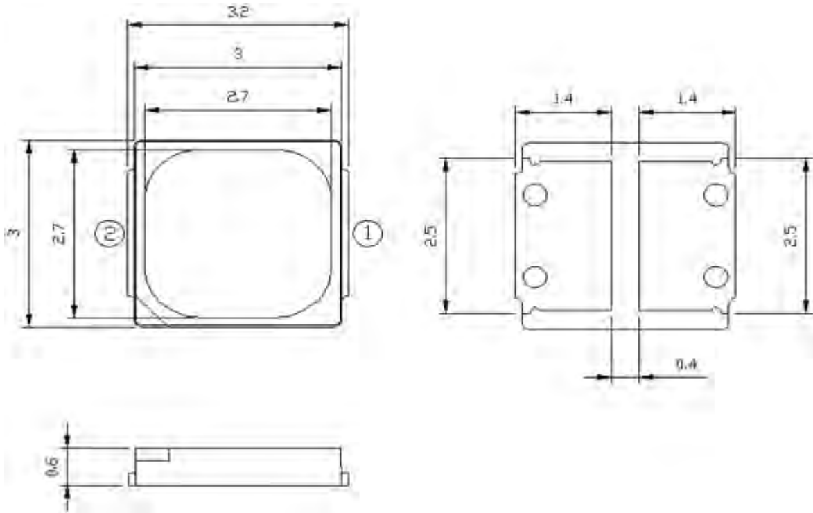
Figure 7 Mechanical Dimensions
