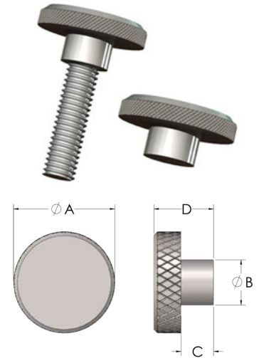
KC1 - KC8 (Course Knurls)
